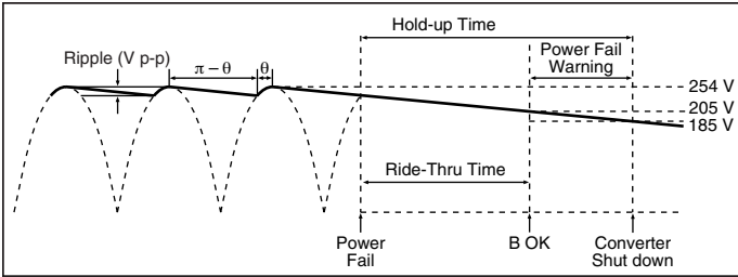
Figure 12—Hold-up time
